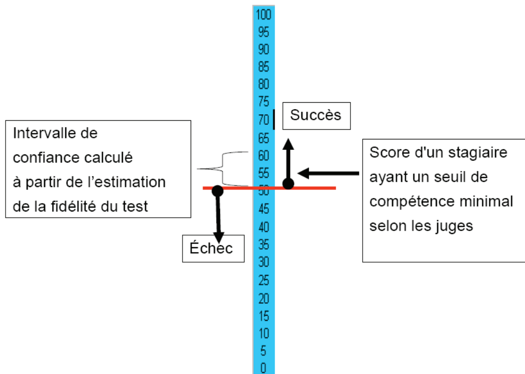
Figure 5.1 Scores seuils
